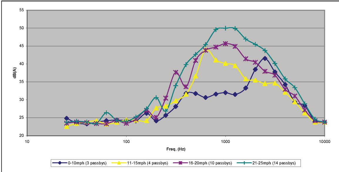
Figure H-6. Th!nk vehicle average L_{max} spectra – cruise (50 ft)
