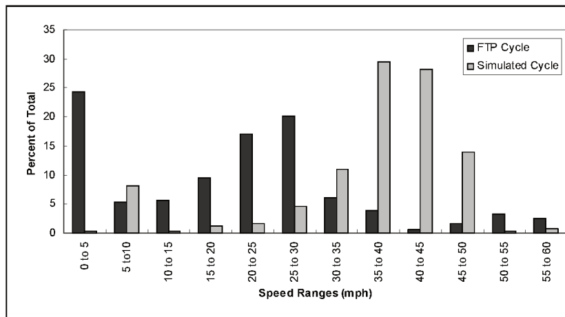
Figure 10. Speed distributions from the FTP and the simulated 1-hour cycle
