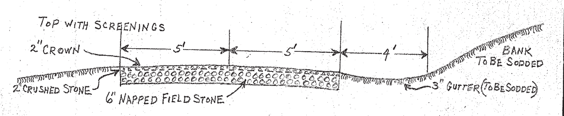
PRESENT DRIVEWAY CROSS SECTION SCALE 3/8" = 1'-0"
